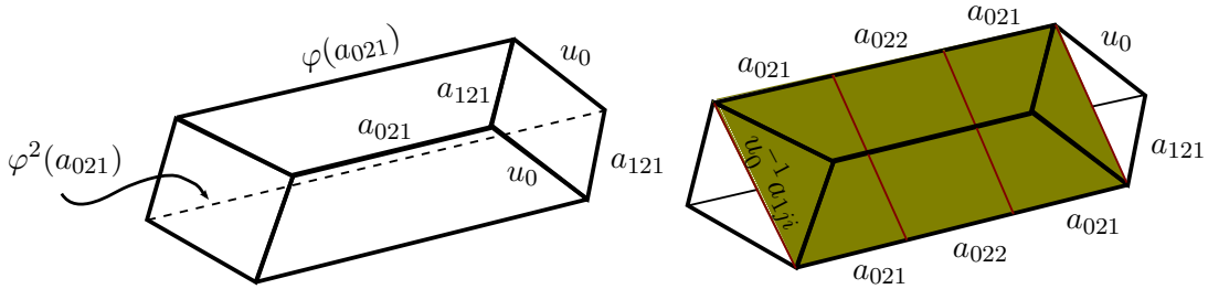
FIGURE 4.3. Typical new 1- and 2-cells in \widetilde{K}_{H_1} .
