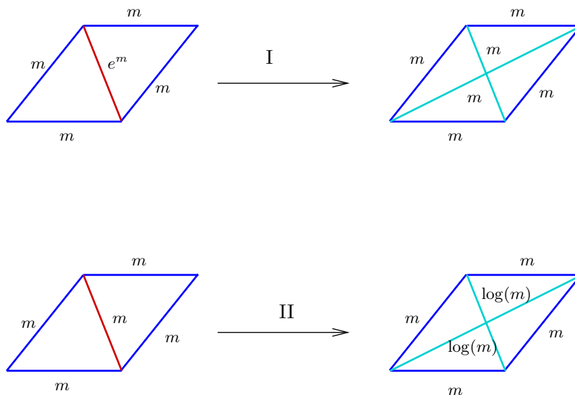
FIGURE 3.4. Geometric versions of the combination-subdivision rule.
