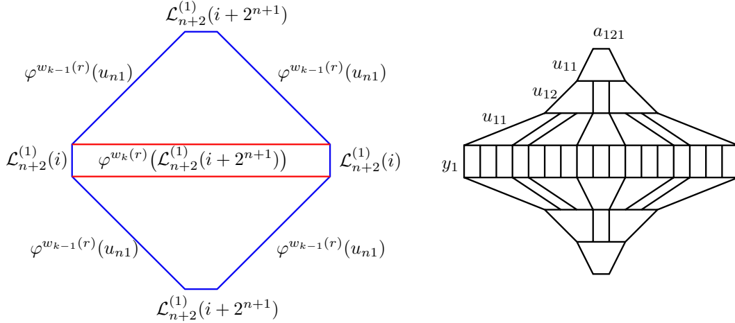
FIGURE 5.5. The van Kampen diagrams \Theta_i^n(w_k(r)) and \Theta_2^1(w_0(1)) .
