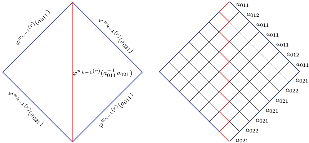
FIGURE 5.4. The van Kampen diagrams \Delta_{12}^0(w_k(r)) and \Delta_{12}^0(w_0(2)) .
