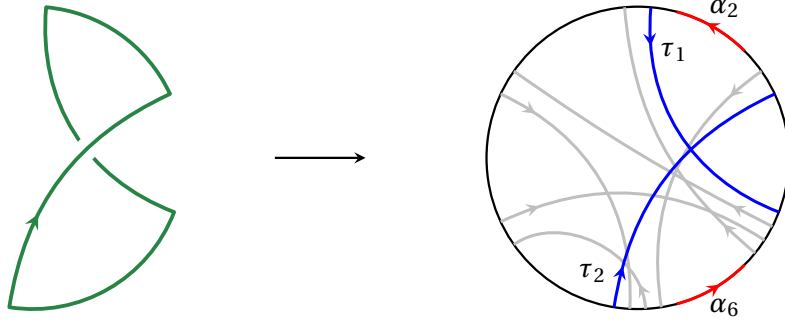
FIGURE 2. A taut turn path in D_1 which runs over \tau_1 , \bar{\alpha}_6 , \tau_2 , and \alpha_2 . Every turn path extends to a map of a disk; in this case the disk is twisted.
