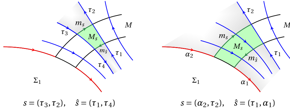
FIGURE 3. Two examples of dual pairs of sides (s, \hat{s}) . Geometrically, each side encodes a portion of the boundary of a possible turn disk (shaded gray in the figure) mapping to D .
